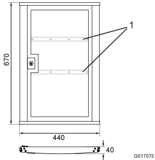
Figure 2. The supporting crossbars (1) can be moved up or down slightly in order to fit the internal equipment.
